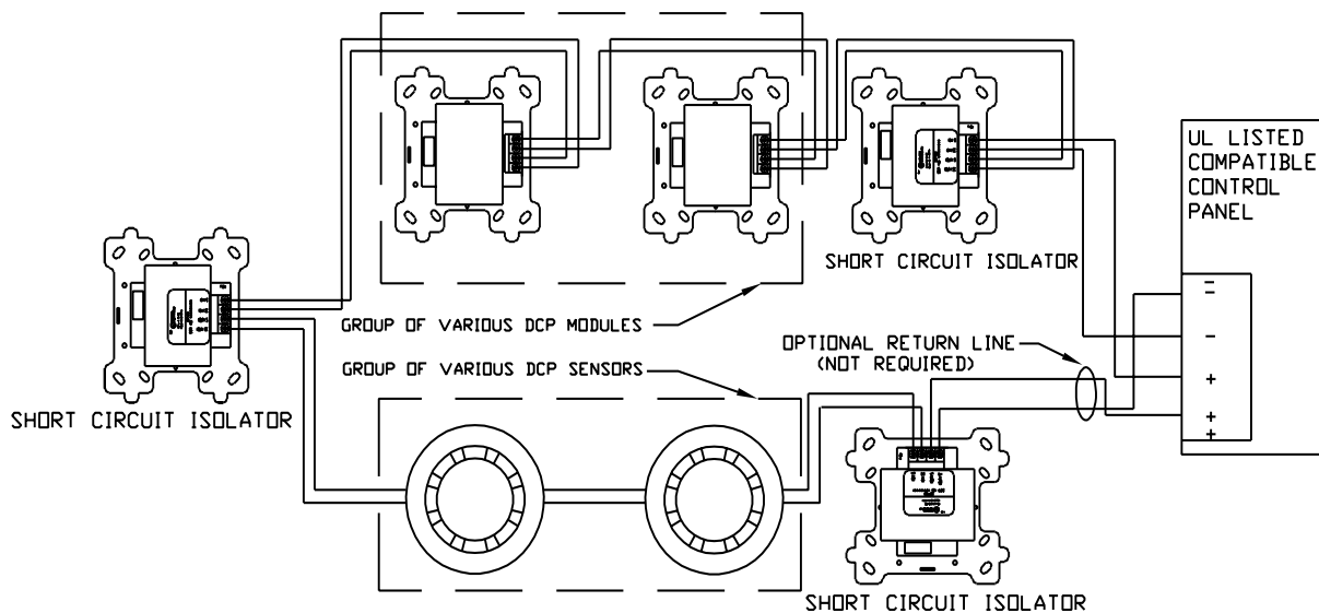
TYPICAL WIRING DIAGRAM EXAMPLE, CONNECTED TO A COMPATIBLE LISTED CONTROL PANEL
