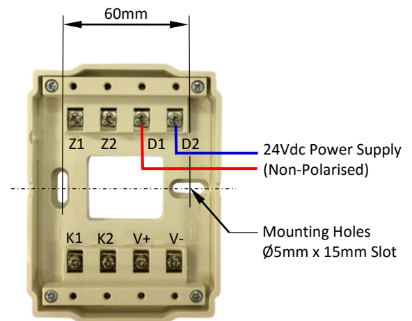
MOUNTING BASE DETAILS
