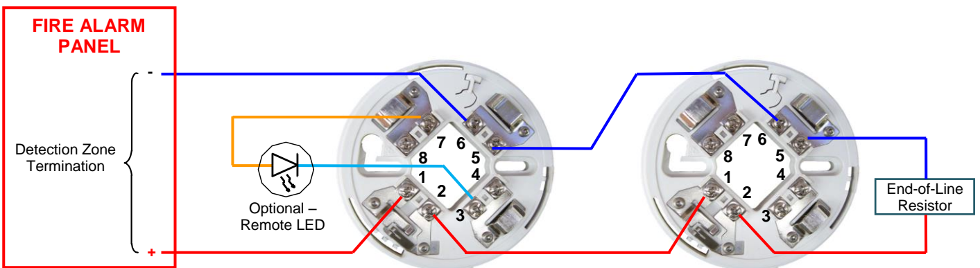
Typical Detector Termination Diagram
